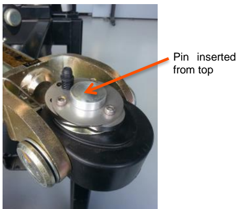
Bi-lock pin installed in DO35 coupling (Top View)
